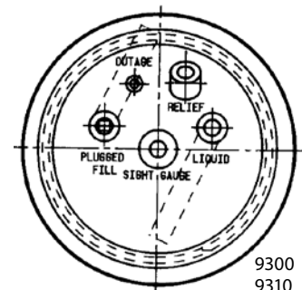
5 Hole Head Plugged Fill Code 13
