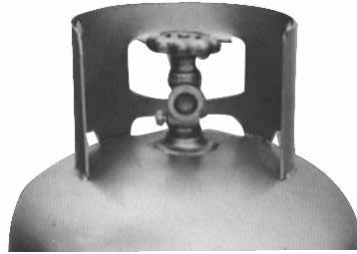
Standard POL Valve CGA510 Connection
